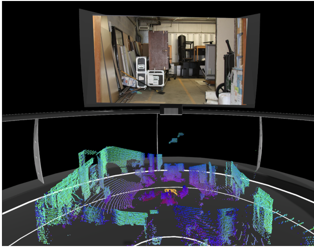
Figure 1: The Cyber-Physical Control Room augmented virtuality HMD interface renders live 3D video streams, a dense 360° 3D point cloud, and a state visualization virtual robot within an immersive virtual environment.
